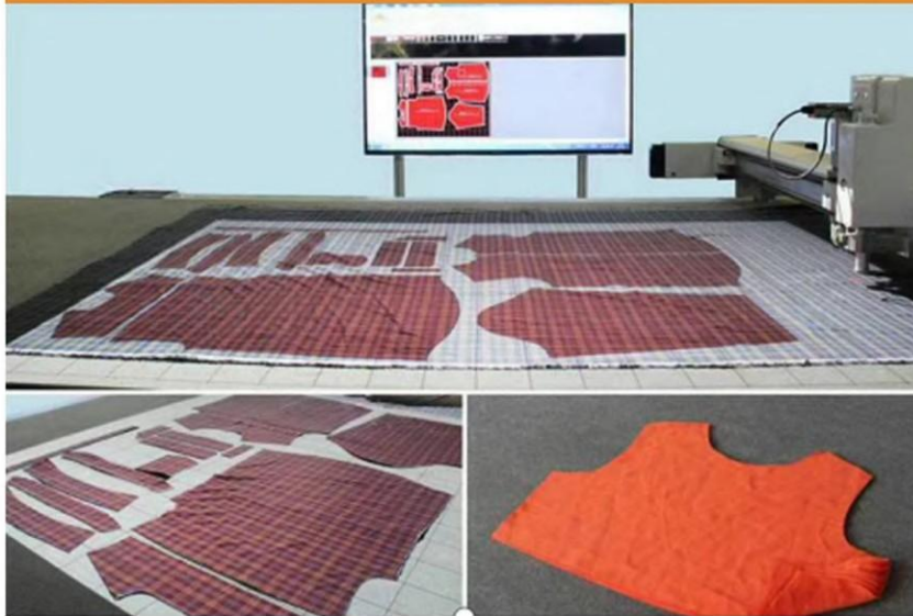
INTEGRATED SOLUTION OF INTELLIGENT CUTTING OF CLOTHING FABRICS
